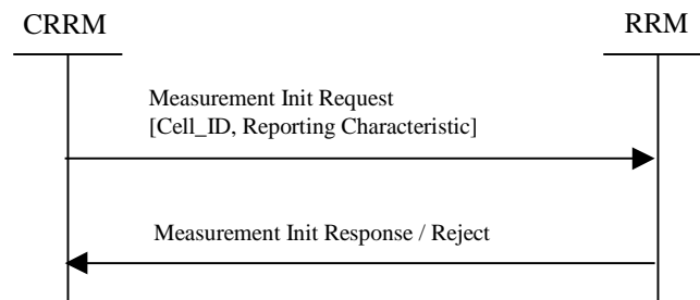
Figure 6: Measurement Initiation Procedure
