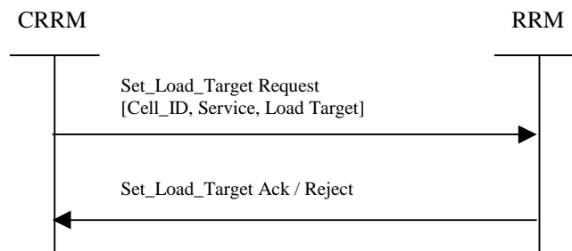
Figure 9: Load Target Setting Procedure
