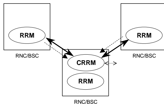
Figure 4: CRRM integrated only in some RNC/BSCs
