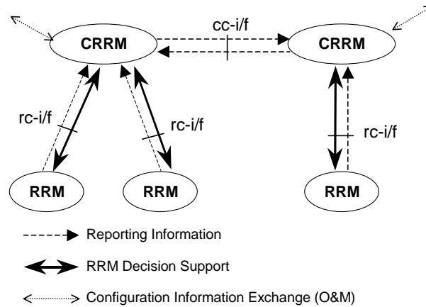
Figure 2: CRRM functional model
